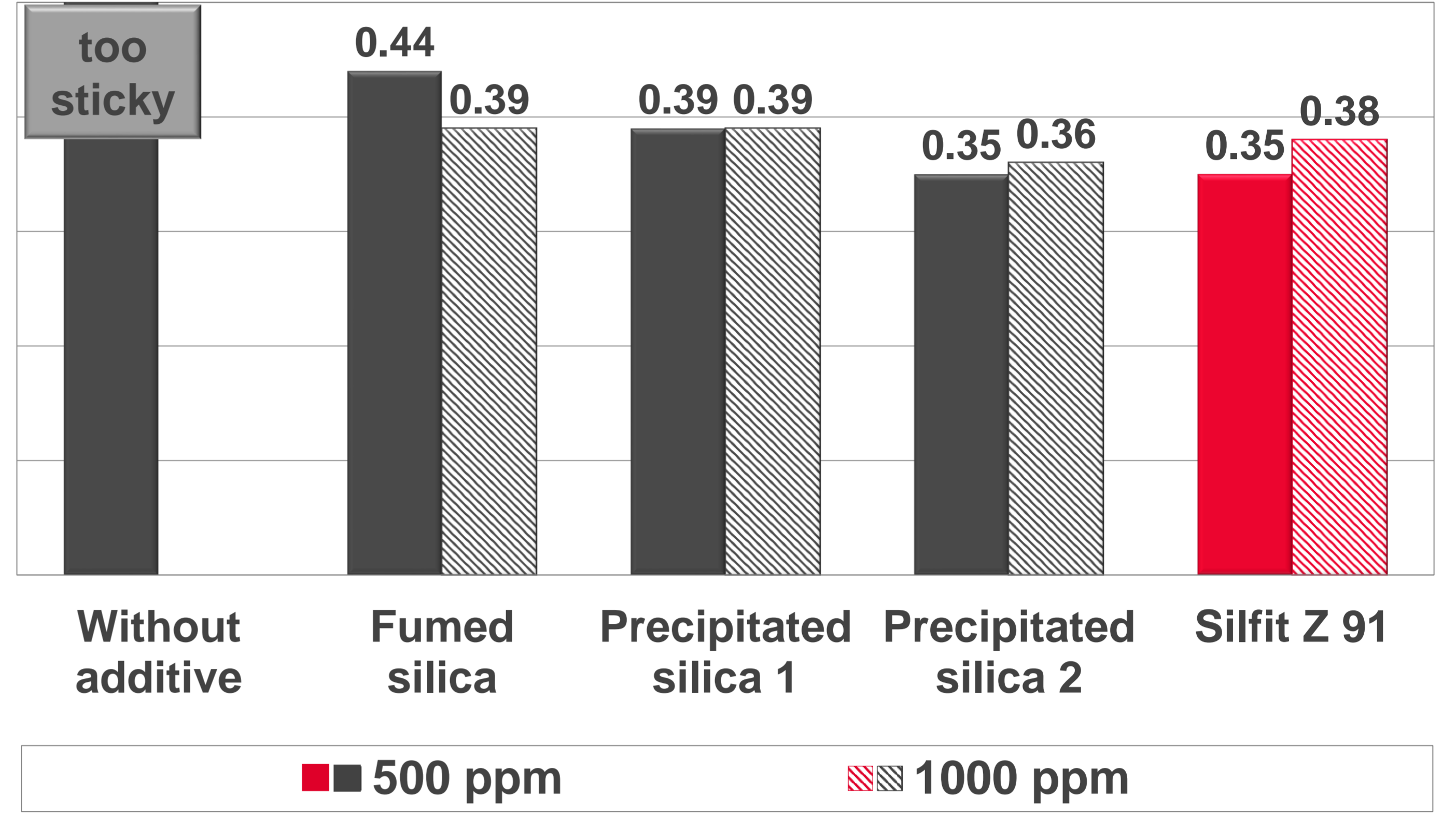
Coefficient of Friction COF [-] Film / Film, static
