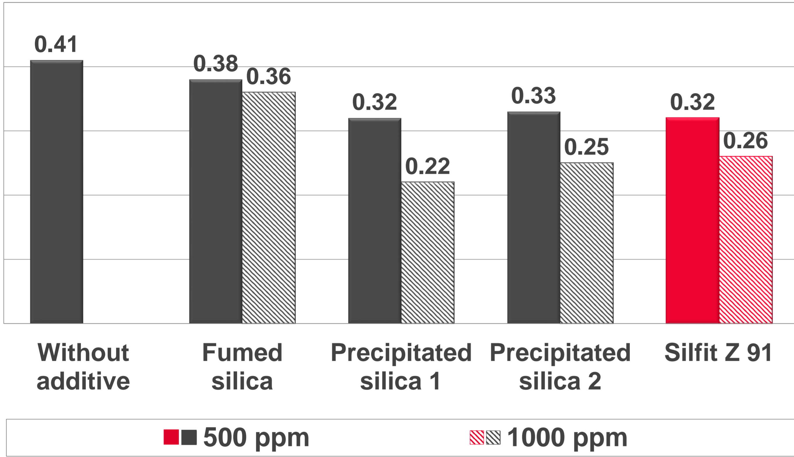
Coefficient of Friction COF [-] Film / Metal, static
