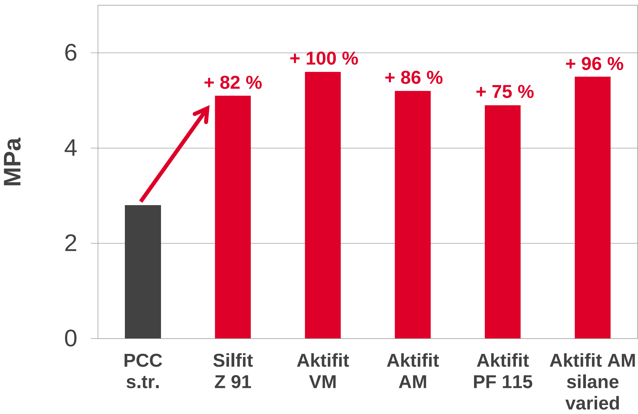
Lap Shear Strength Aluminum, 28d, 1 mm
