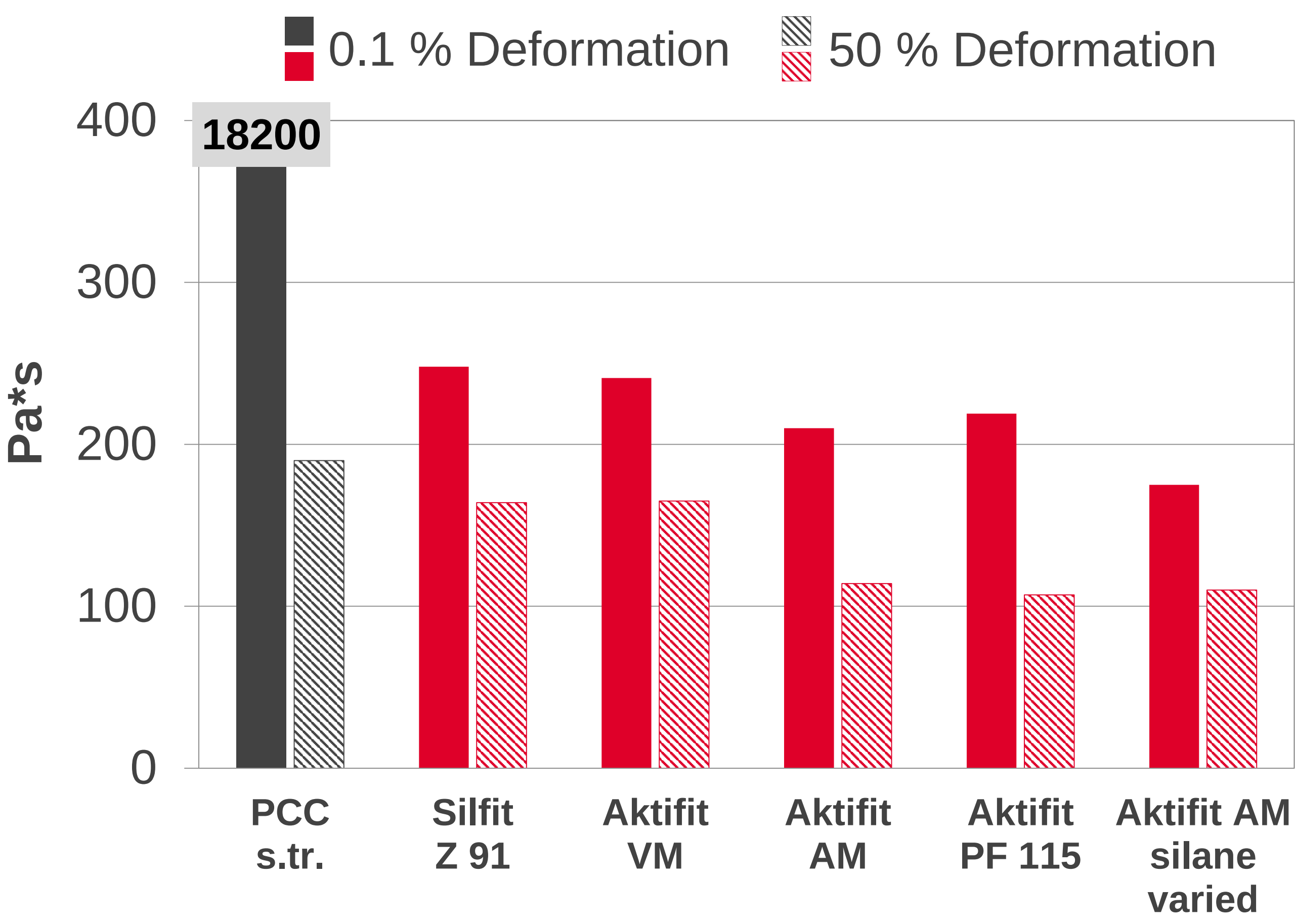
Complex Viscosity
