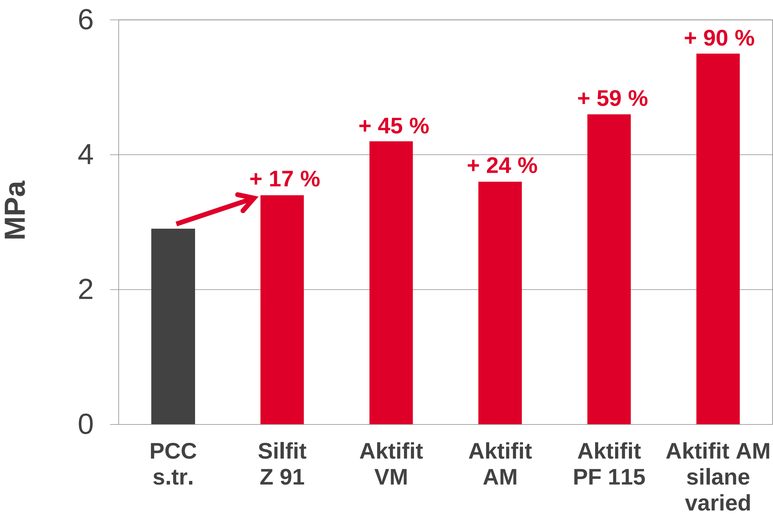
Lap Shear Strength Beech Wood, 28d, 1 mm
